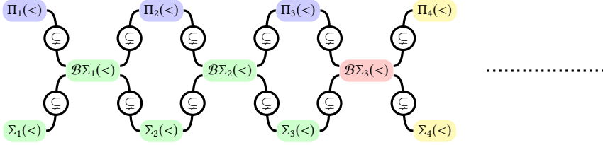
Fig. 1. Quantifier alternation hierarchy within \text{FO}(<) .
