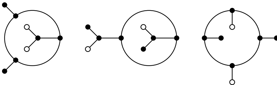
Figure 9: Hurwitz generation of \mathrm{PSL}_2(13) .
