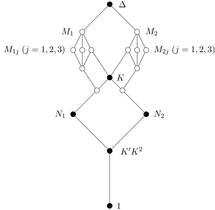
Figure 14: The subgroups M_{ij} of \Delta (normal and non-normal subgroups are indicated in black and white)
