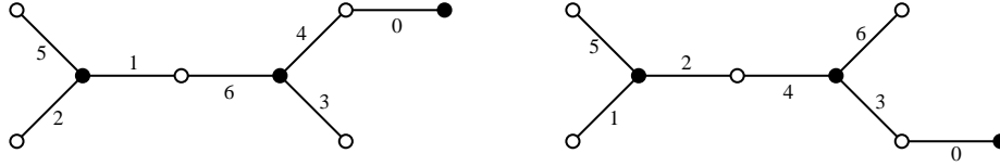
Figure 2: Trees providing a (3, 2, 7) -generation of the group \text{PSL}_3(2) .
