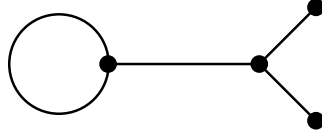
Figure 4: A map with the monodromy group \mathrm{PSL}_2(7) . White vertices in the middle of the edges are implicit.
