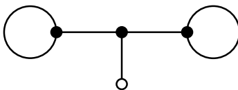
Figure 7: A map with monodromy group \mathrm{PSL}_2(8) .
