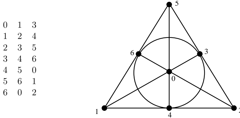
Figure 1: The Fano plane.
